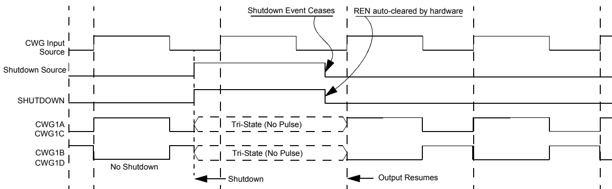
Figure 25-18. SHUTDOWN FUNCTIONALITY, AUTO-RESTART ENABLED (REN = 1, LSAC = 01, LSBSD = 01)
