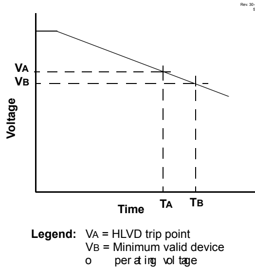
Figure 35-4. Typical Low-Voltage Detect Application
