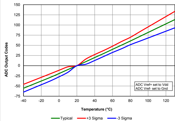
Figure 41-88. Temperature Indicator, Slope Normalized to 20°C, High Range, VDD = 5.5V, PIC18F67K40 only
