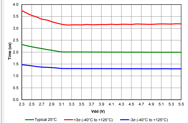
Figure 41-10. ADC RC Oscillator Period, PIC18F67K40 only
